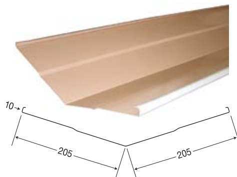
VALLEY GUTTER Rollformed
